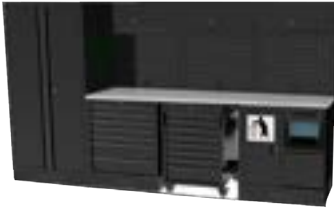
SPUSS222S - STAINLESS STEEL TOP €5550 SPUSS222W - WOODEN TOP €5250 3490B X 660D X 2000H MM
