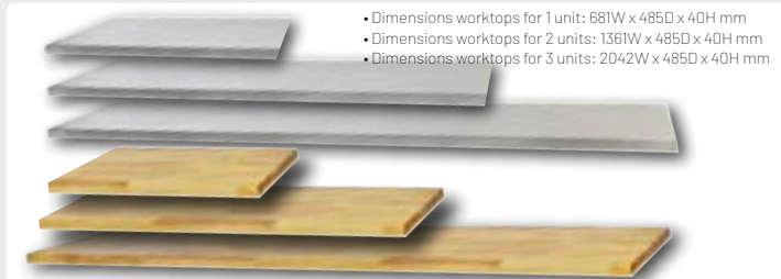
SP WORKSHOP SERIES WORKTOPS: LUXURY SOLID RUBBERWOOD OR STAINLESS STEEL FOLDED • Dimensions worktops for 1 unit: 681W x 485D x 40H mm • Dimensions worktops for 2 units: 1361W x 485D x 40H mm • Dimensions worktops for 3 units: 2042W x 485D x 40H mm SP41150 RUBBER WOOD TOP FOR 1 UNIT (40MM) €139 SP41160 STAINLESS STEEL FOLDED TOP FOR 1 UNIT (40MM) €125 SP41151 RUBBER WOOD TOP FOR 2 UNITS (40MM) €229 SP41161 THICK STAINLESS STEEL FOLDED TOP FOR 2 UNITS (40MM) €219 SP41155 RUBBER WOOD TOP FOR 3 UNITS (40MM) €349 SP41165 STAINLESS STEEL FOLDED TOP FOR 3 UNITS (40MM) €299
